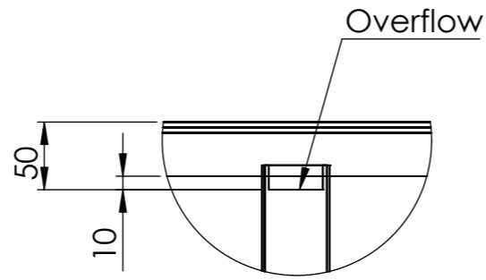
DETAIL B SCALE 1 : 5
